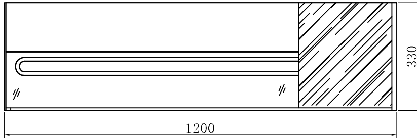
1200 330 Over Look View 俯视图
