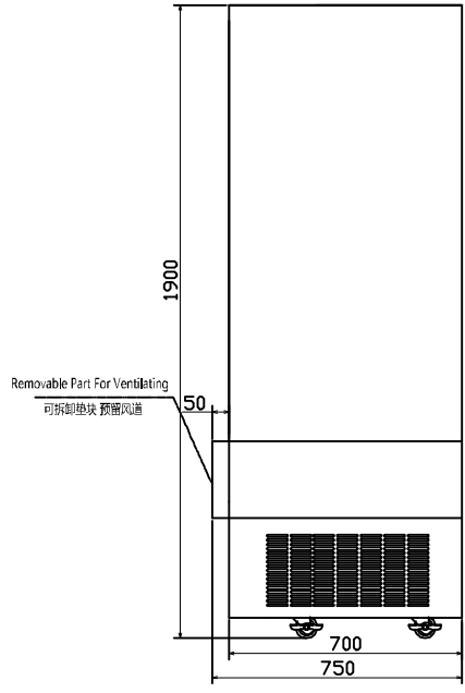
Left Side View 左侧视图
