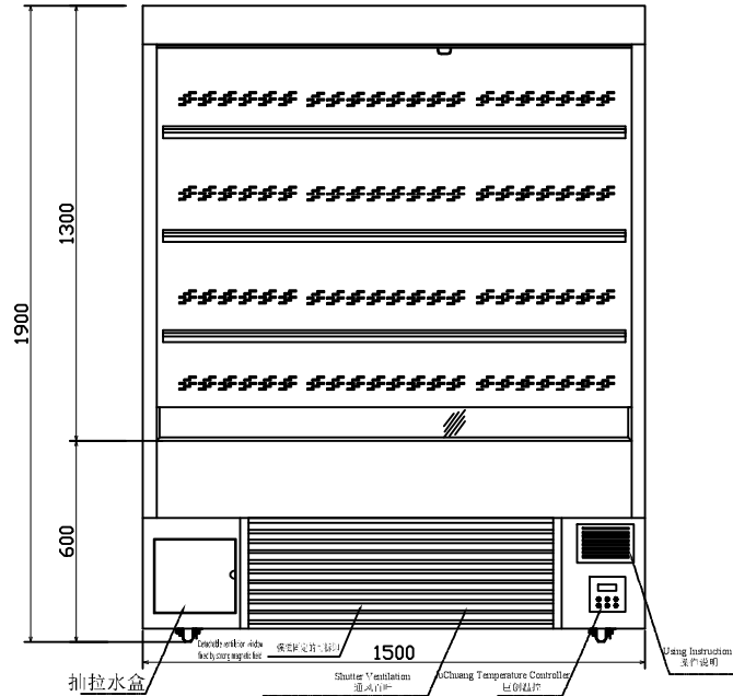
Front Look View 正视图
