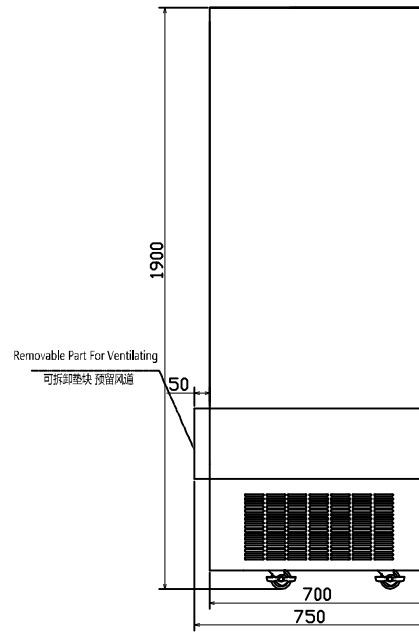
Left Side View 左侧视图
