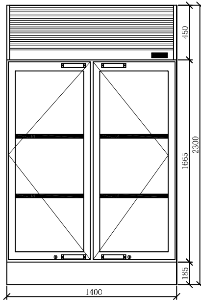
Front Look View 正视图
